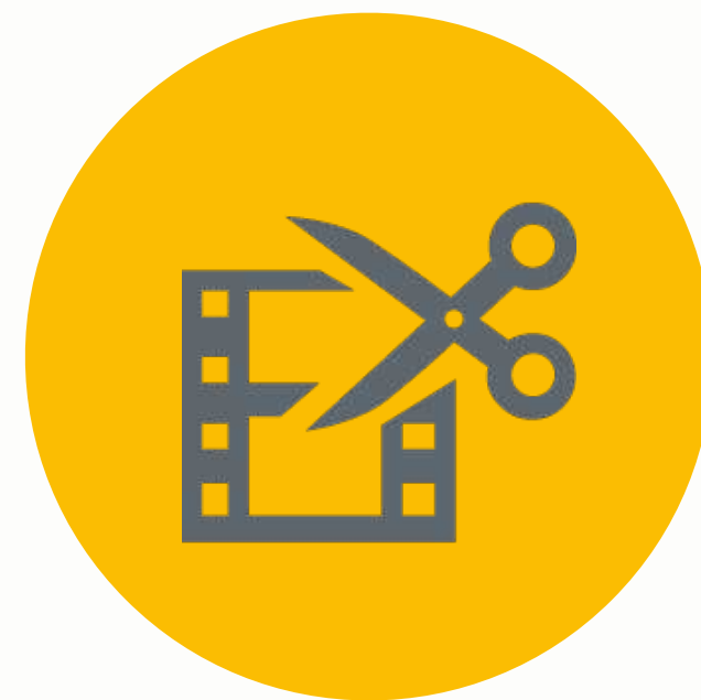
Video Editing
