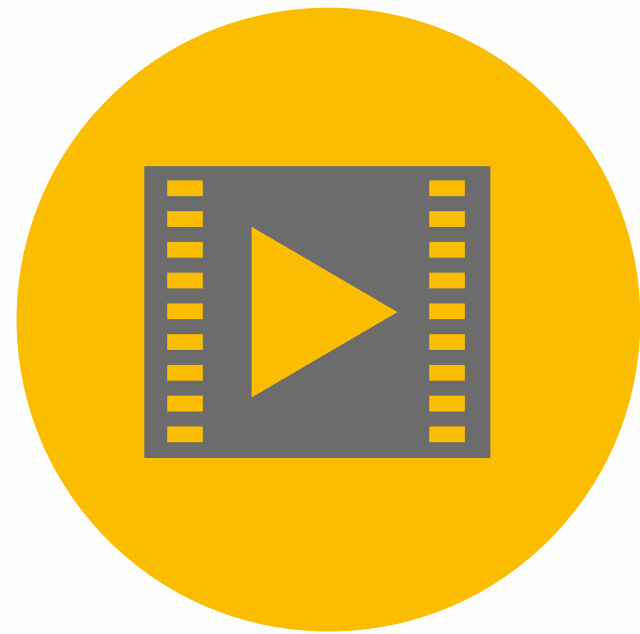
Video Production
